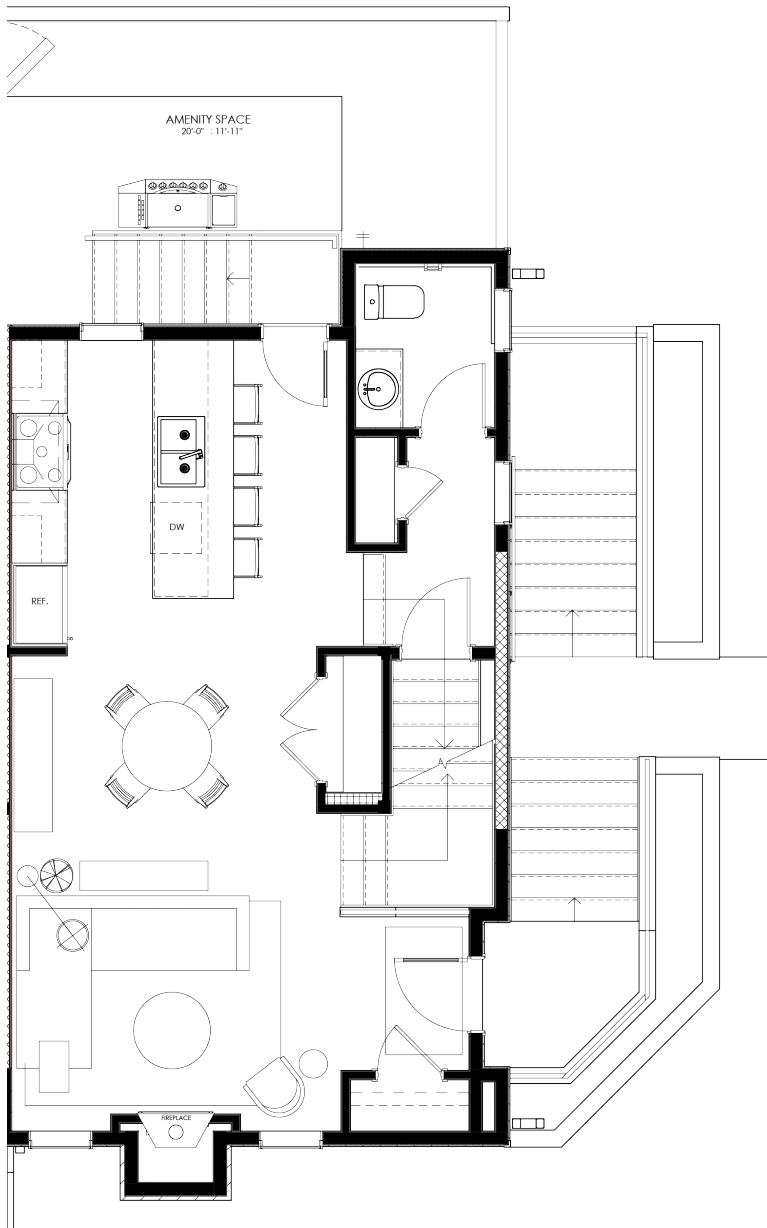
MAIN LEVEL
