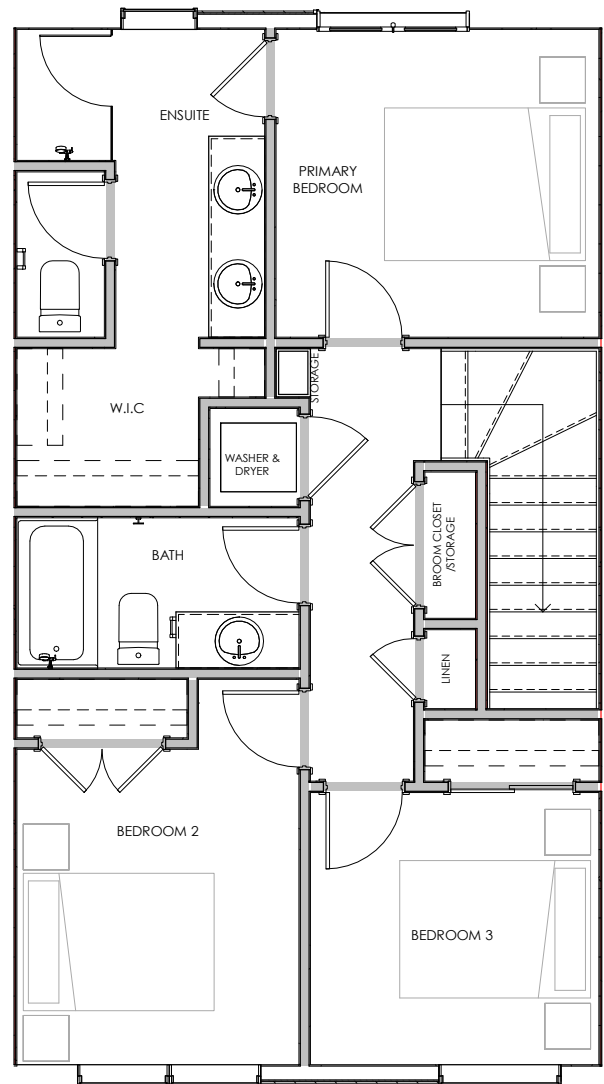
UPPER LEVEL
